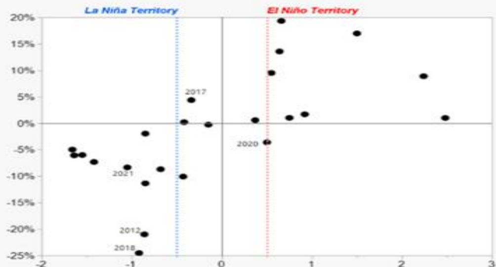
Argentina Corn Yields and ENSO, since 1997/98 Yield deviation from trend (Y-axis) vs. Niño 3.4 SST anomaly (°C), Dec-Feb (X-axis)
